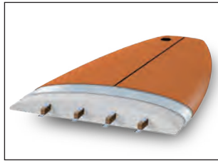
Bamboo stringers(image shows 10") 7'0" (2) / 8'4" (3) / 10'0" (4)
